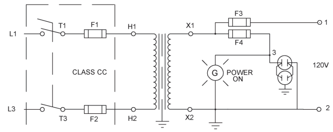
BASE UNIT WITH FUSED DUPLEX RECEPTACLE OPTION
