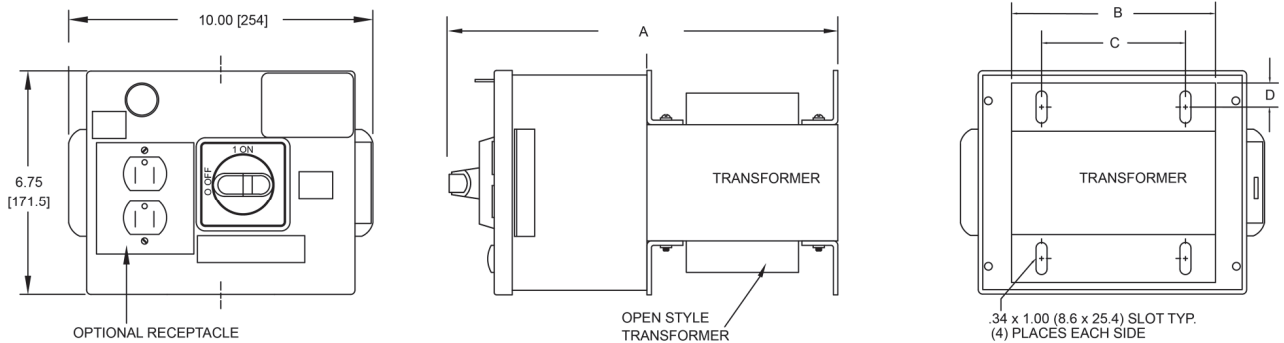
ALL DIMENSIONS ARE IN INCHES AND [MM]
