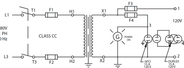
BASE UNIT WITH (2) GFI PROTECTED RECEPTACLES OPTION
