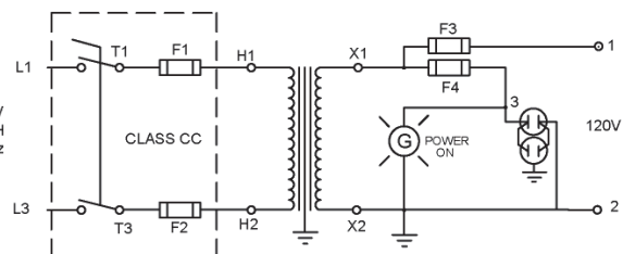
BASE UNIT WITH FUSED RECEPTACLE OPTION
