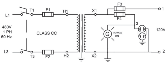
BASE UNIT WITH FUSED DUPLEX RECEPTACLE OPTION
