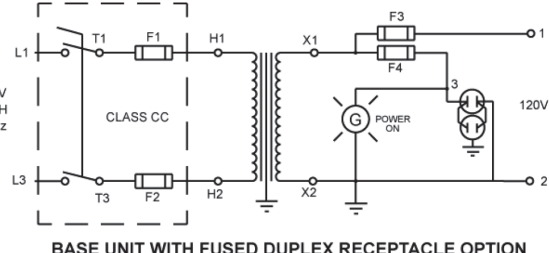
BASE UNIT WITH FUSED DUPLEX RECEPTACLE OPTION
