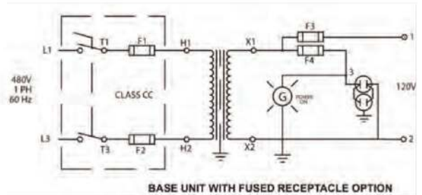
BASE UNIT WITH FUSED RECEPTACLE OPTION
