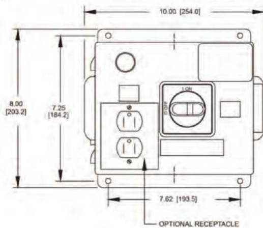
ALL DIMENSIONS ARE IN INCHES AND [MM]
