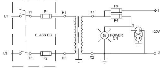
BASE UNIT WITH FUSED DUPLEX RECEPTACLE OPTION
