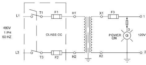
BASE UNIT
