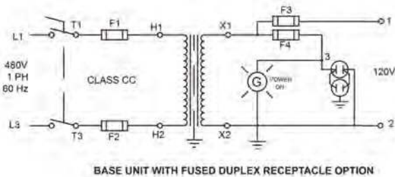
BASE UNIT WITH FUSED DUPLEX RECEPTACLE OPTION
