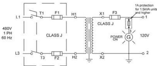
BASE UNIT
